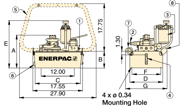
2.6, 5.2, 10.3 gallon reservoirs
