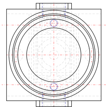
Bottom screw detail
