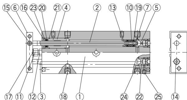
CXSM15
