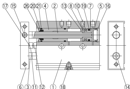
CXSM15
