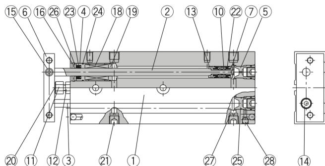
Parts list: Standard piping
