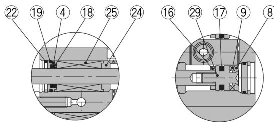
Rod cover
