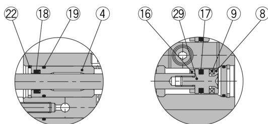
Rod cover
