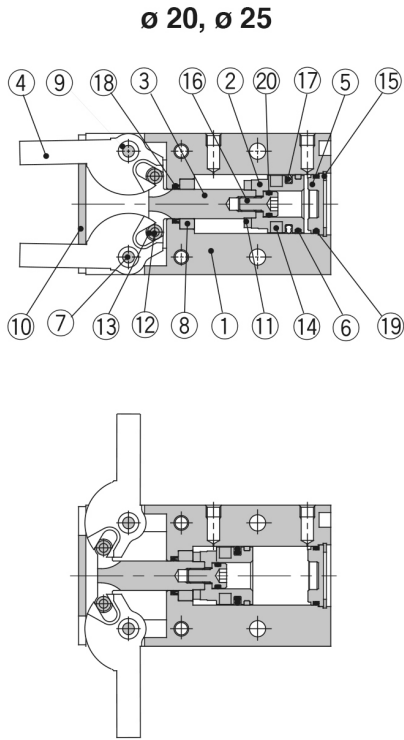
Component Parts
