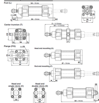
Dimensions: Cylinder Mounting Accessories First angle projection
