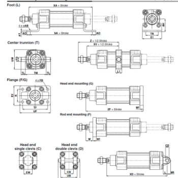
Dimensions: Cylinder Mounting Accessories (First angle projection)
