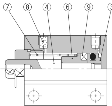
Built-in magnet
