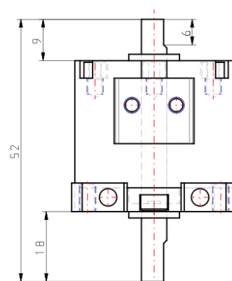
Detail shaft W
