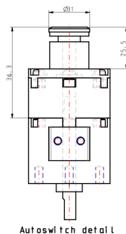
Autoswitch detail
