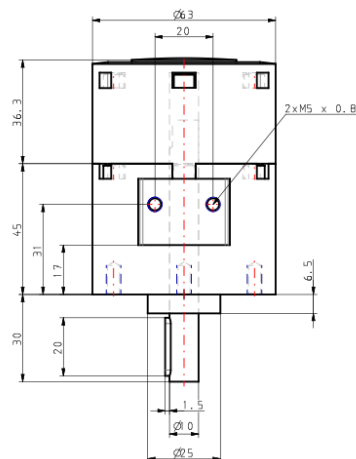
Autoswitch detail
