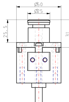
Autoswitch detail
