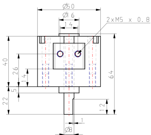
Flange detail
