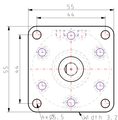
Flange detail
