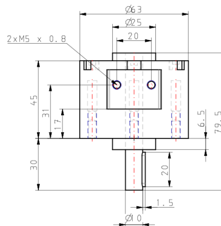
Autoswitch detail
