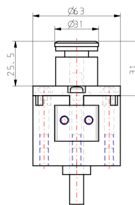
Autoswitch detail
