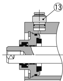
Built-in one-touch fittings
