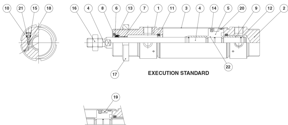
AIMANT INTEGRE
