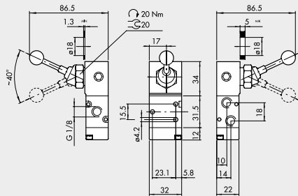
90°- HEBEL 3/2 1/8"
