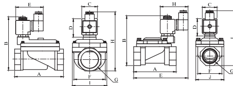
Dimensions (mm)
