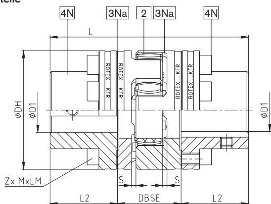
Bauart AFN
