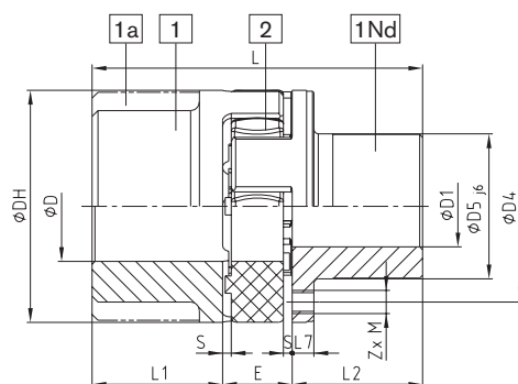
Bauart FNN
