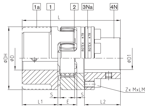
Bauart BFN
