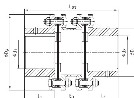
Bauart NANA 2
