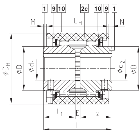
Bauart AS
