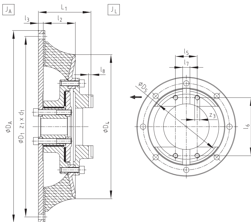
Bauart HEG2
