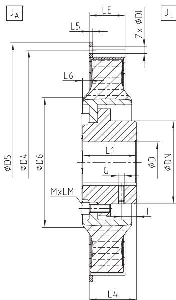
Bauart AK
