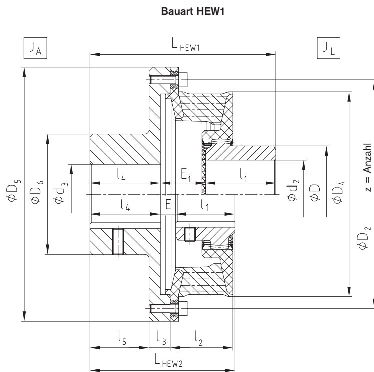
Bauart HEW2
