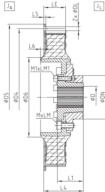
Bauart ALC
