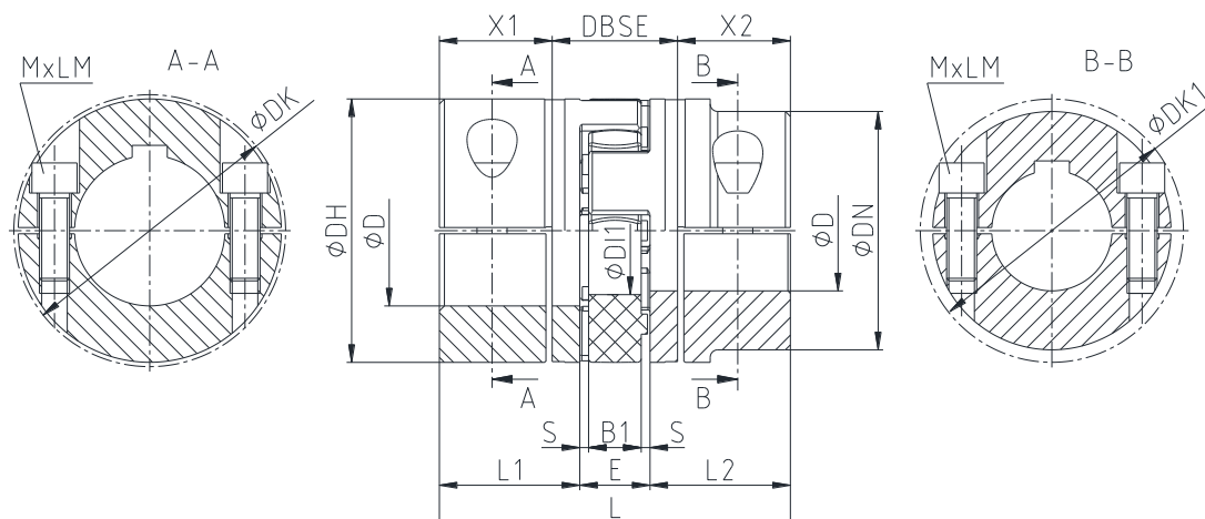
Illustration 1: ROTEX® type AH (material: steel)
