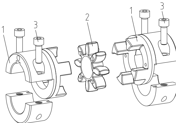
Illustration 3: ROTEX® type AH, size 19 - 90
