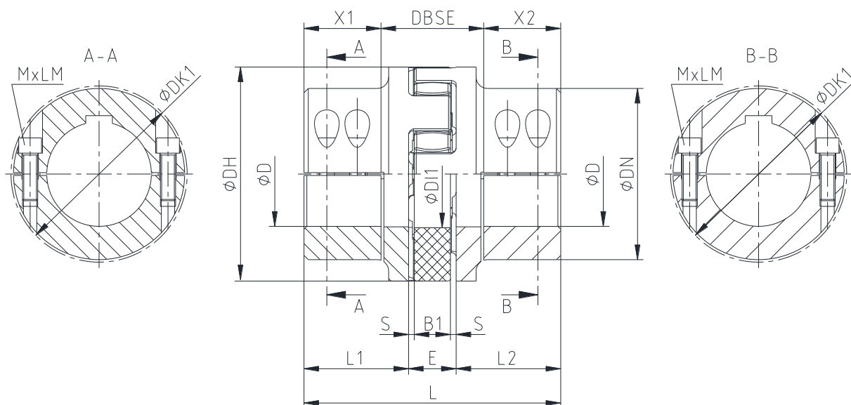
Illustration 2: ROTEX® type AH (material: EN-GJS-400-15)
