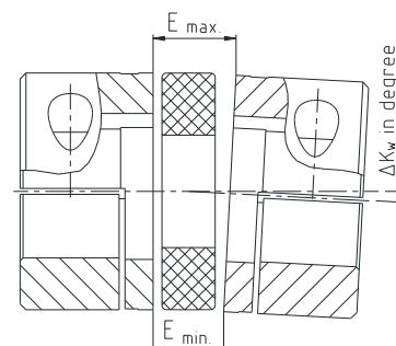
Angular displacements
