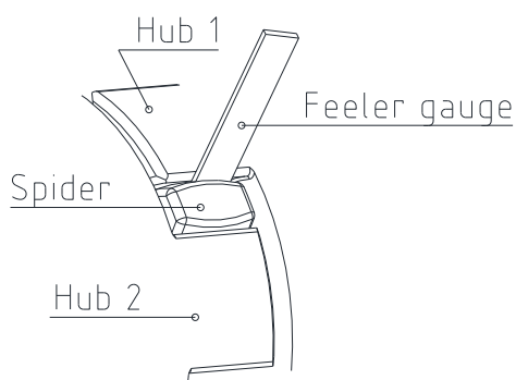
Illustration 14: Inspection of the limit of wear
