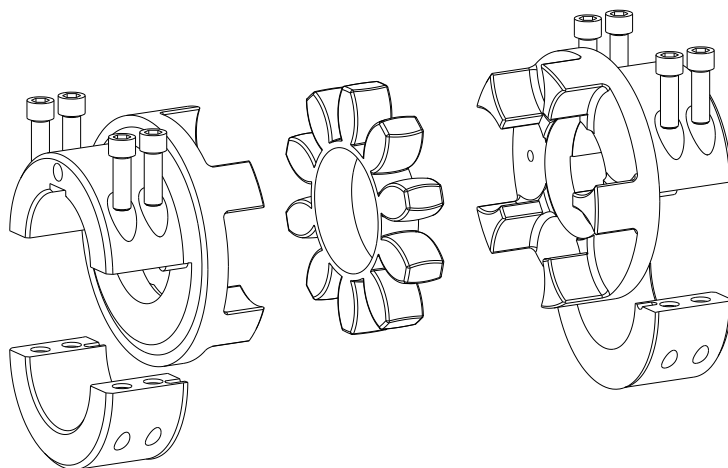
Type AH, Size 100 - 180
