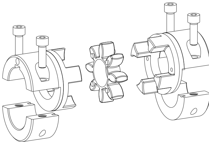
Type AH, Size 19 - 90
