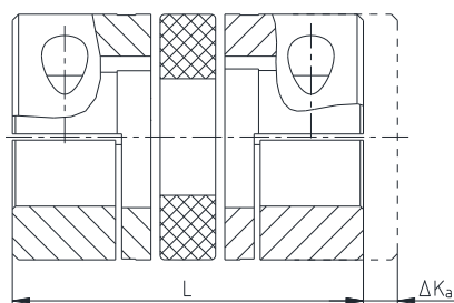
Axial displacements
