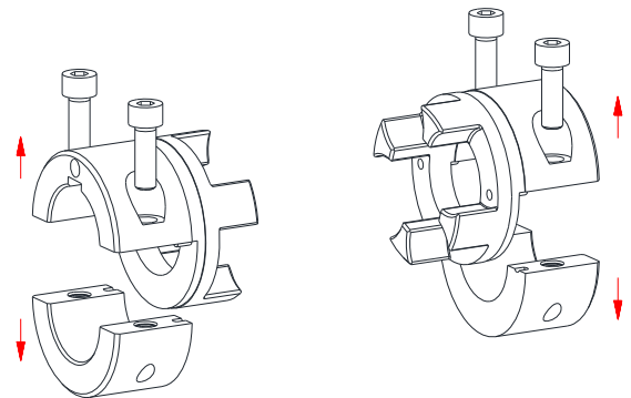
Illustration 6: Disassembly of shells
