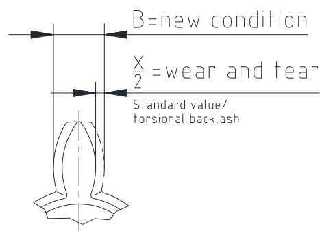
Illustration 15: Wear of spider
