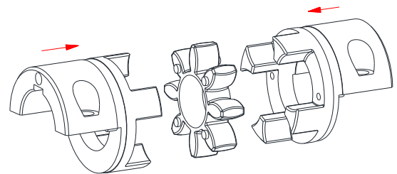
Illustration 7: Assembly of hub bodies, spiders and DKM-H spacer
