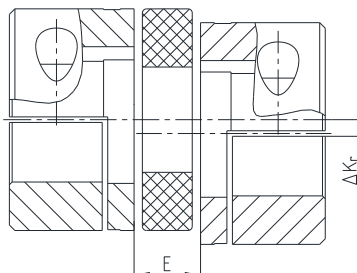
Radial displacements
