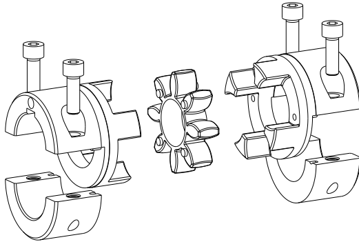
Illustration 12: ROTEX® type AH
