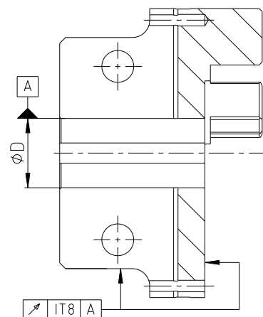
Illustration 5: Concentricity and axial runout
