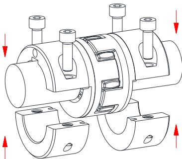
Illustration 8: Assembly of subassembly on the shafts
