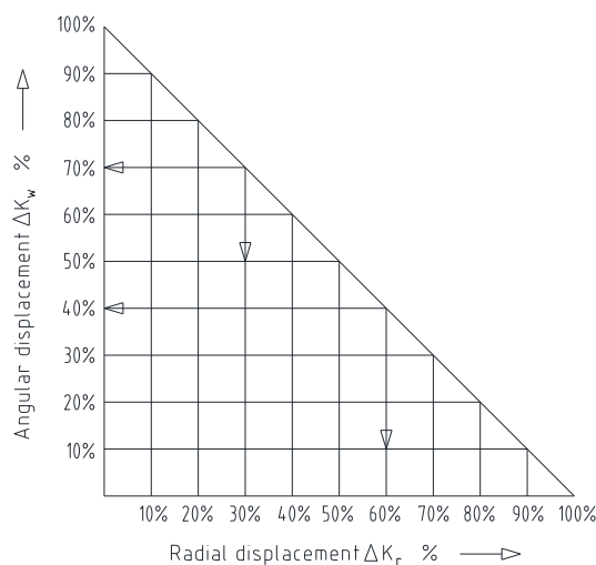
Illustration 11: Combinations of displacement
