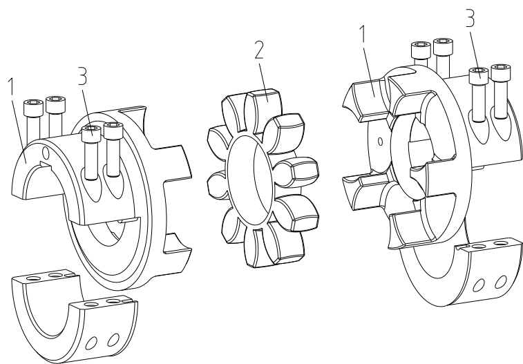
Illustration 4: ROTEX® type AH, size 100 - 180
