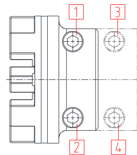
Illustration 9: Tightening of screws
