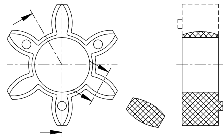
Illustration 13: ROTEX® spider
