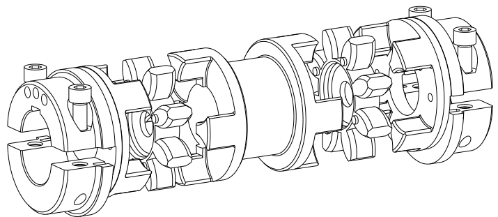
Bauart ZS-DKM-H
