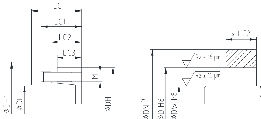
Illustration 2: Dimensions of CLAMPEX® KTR 206
