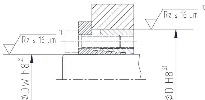
Illustration 3: Tolerances and surfaces (example: CLAMPEX® KTR 206)
