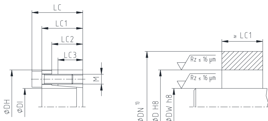
Illustration 1: Dimensions of CLAMPEX® KTR 203
