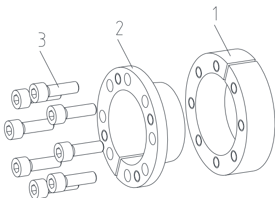
Illustration 4: CLAMPEX® KTR 203
