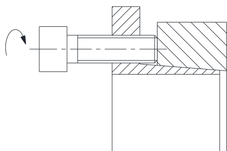
Illustration 9: Releasing the clamping set KTR 206
