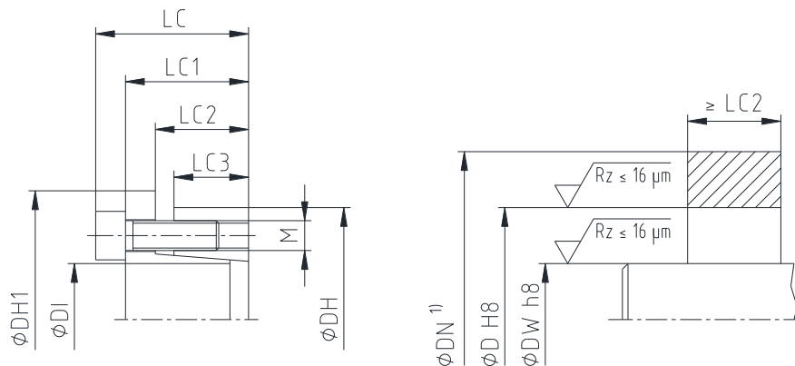
Illustration 2: Dimensions of CLAMPEX® KTR 206
