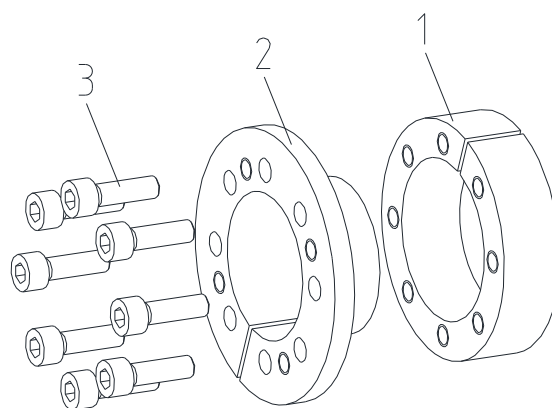
Illustration 5: CLAMPEX® KTR 206
