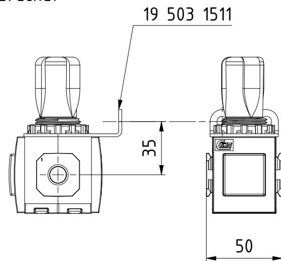
19 503 1511 - Top-mounting ring and bracket
