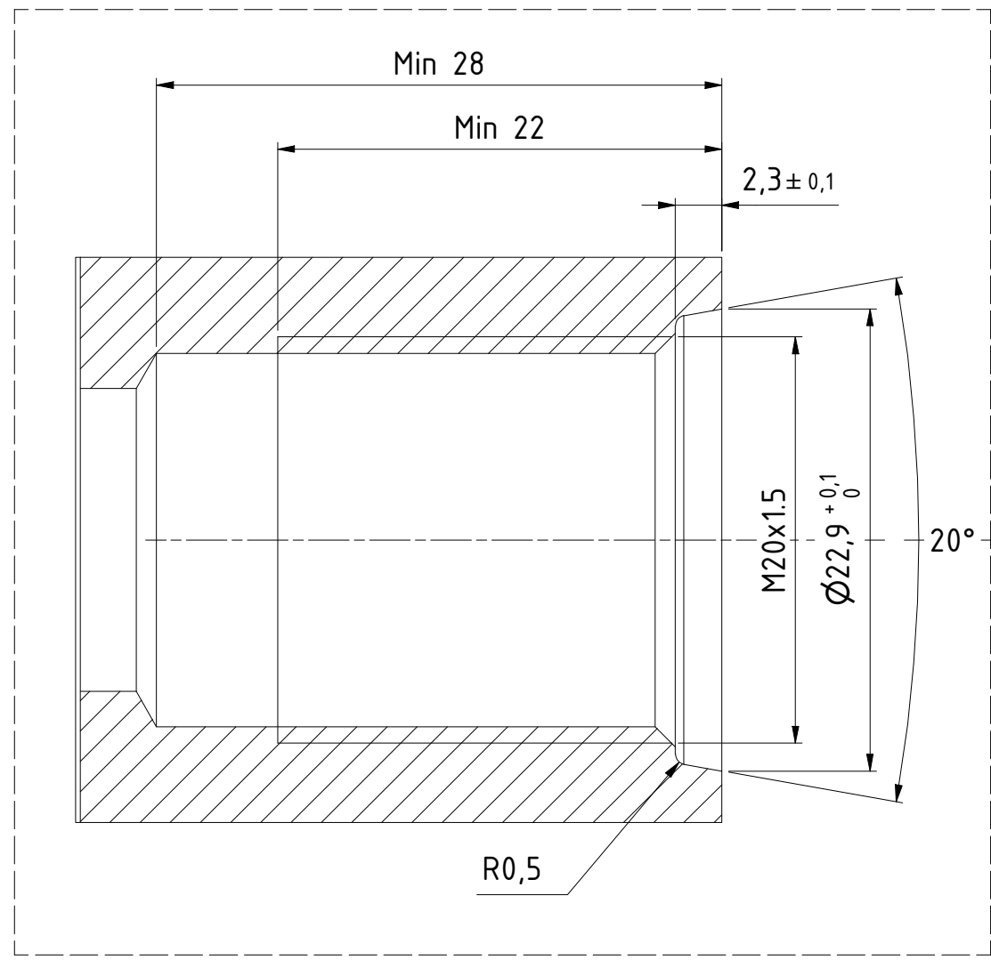
Manifold dimensions
