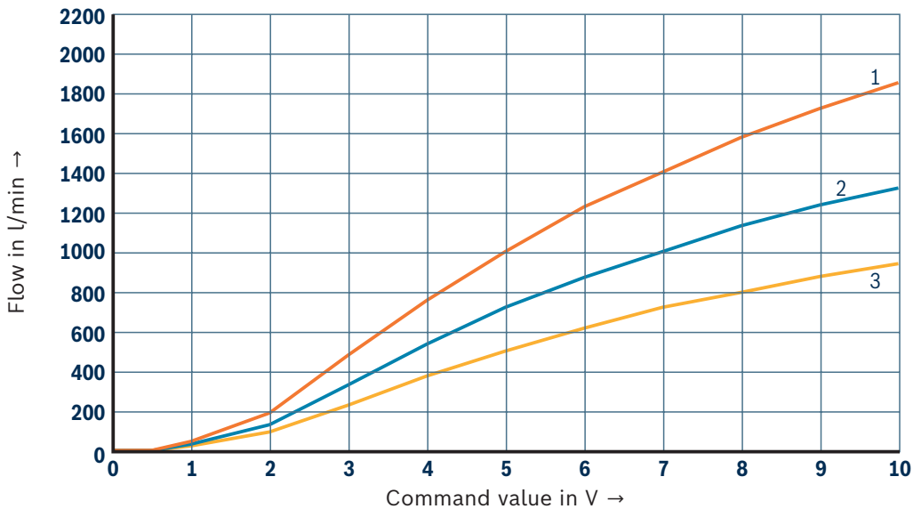
Version "940" (A→B; B→A; linear-progressive)
