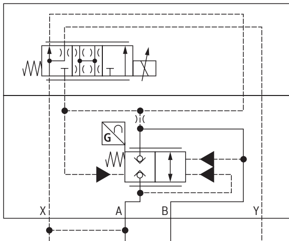
Internal pilot oil supply (A→B)
