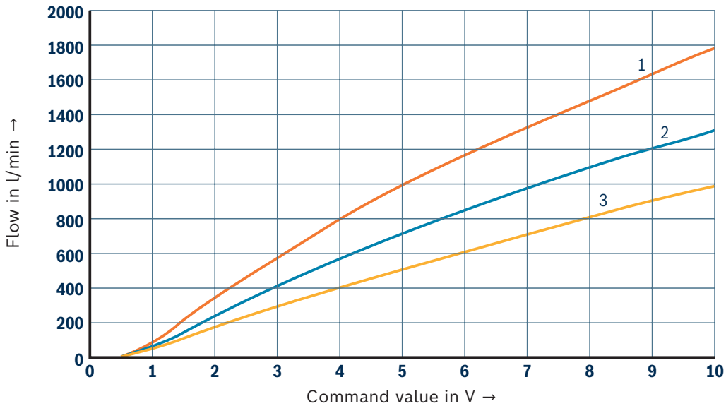
Version "1000" (A→B; B→A; linear)
