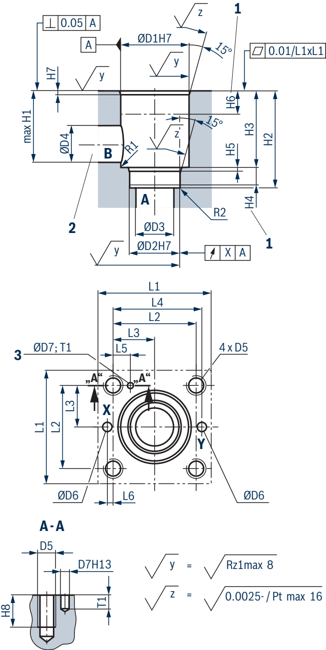
Installation dimensions according to ISO 7368
