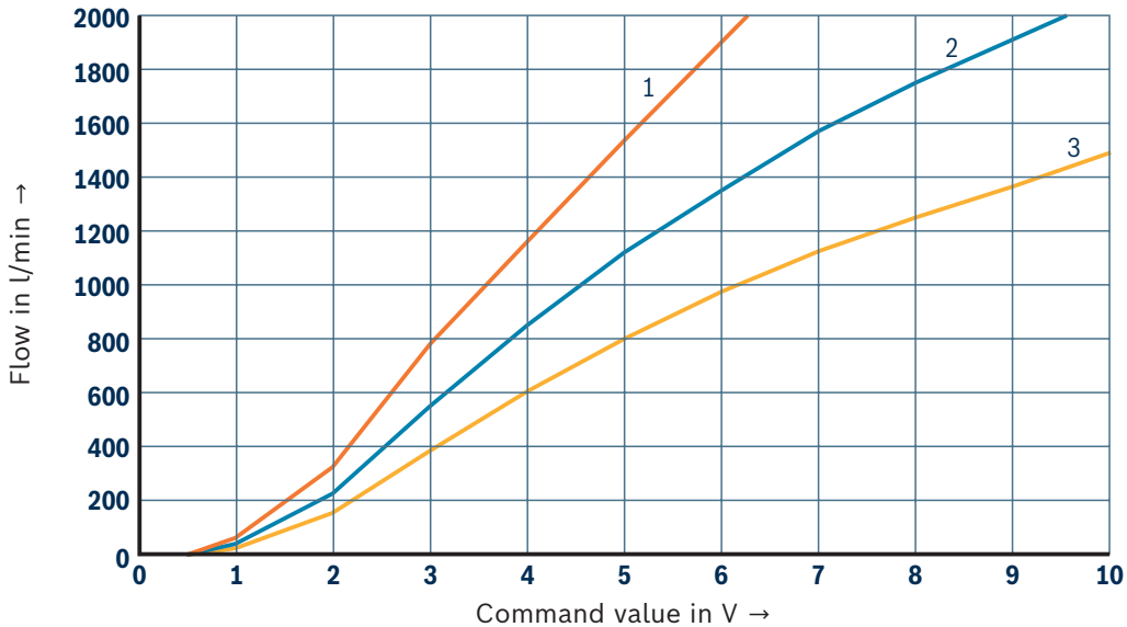
Version "1500" (A→B; B→A; linear-progressive)
