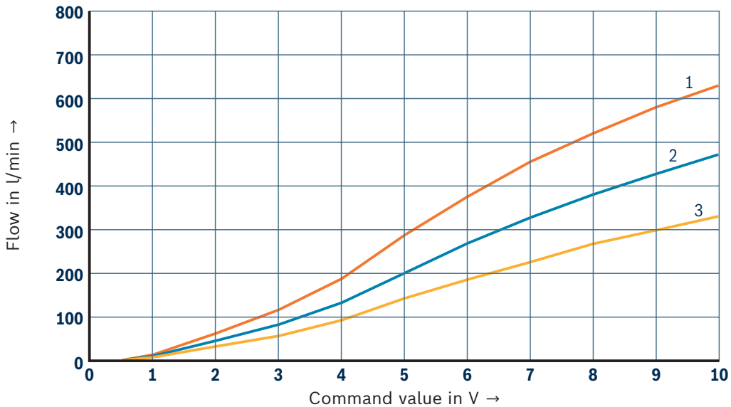
Version "330" (A→B; B→A; linear-progressive)
