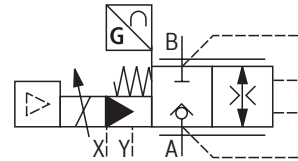
Integrated electronics (OBE) "2WFCE"
